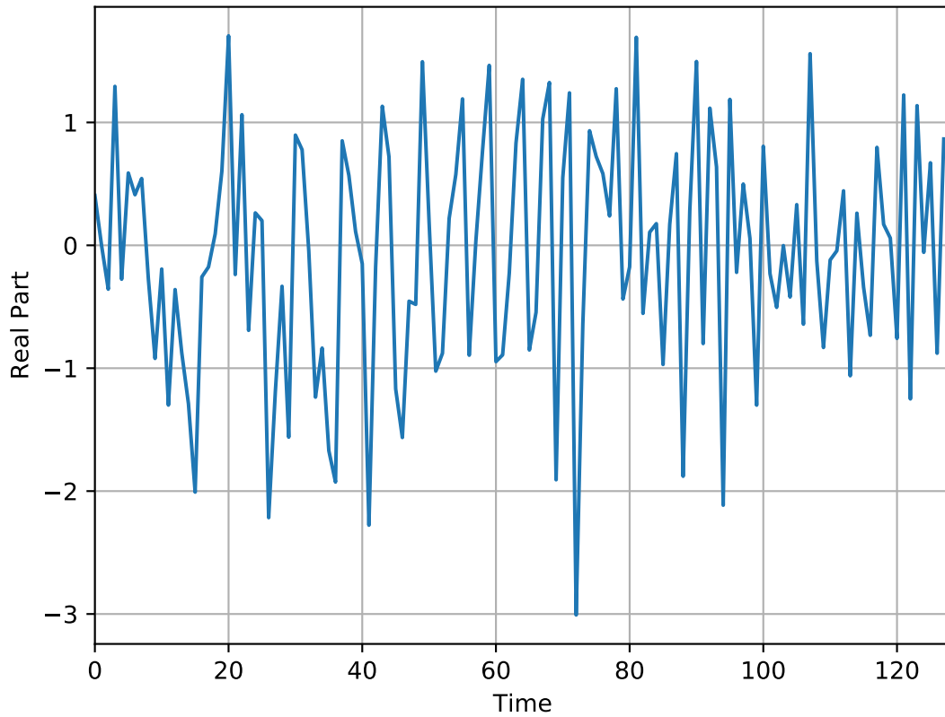
Noisy chirp
