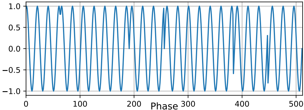
Analytic QPSK signal
