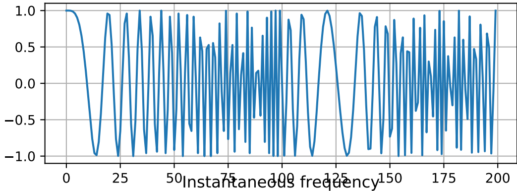
Linear and Sinusoidal modulated signal
