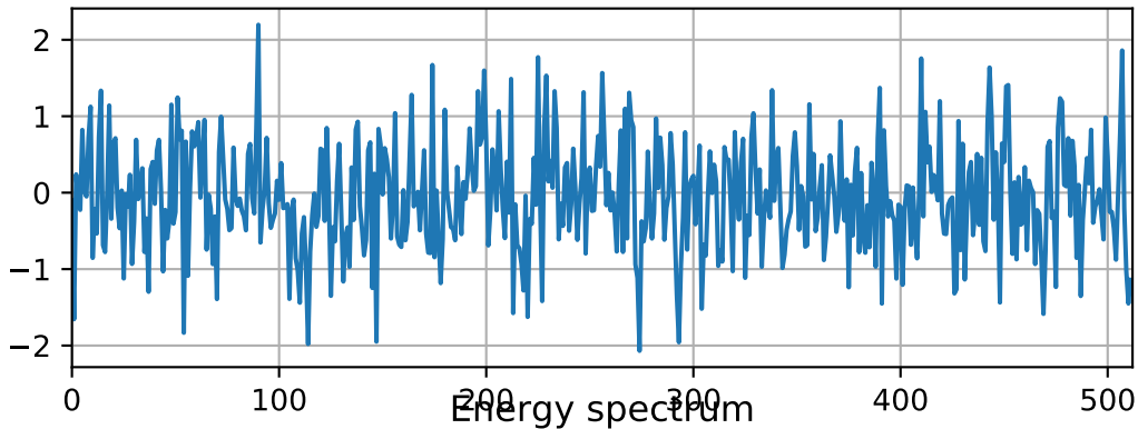
Analytic complex Gaussian noise.
