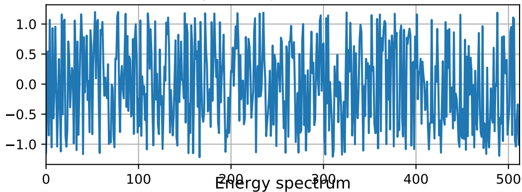
Analytic complex white noise
