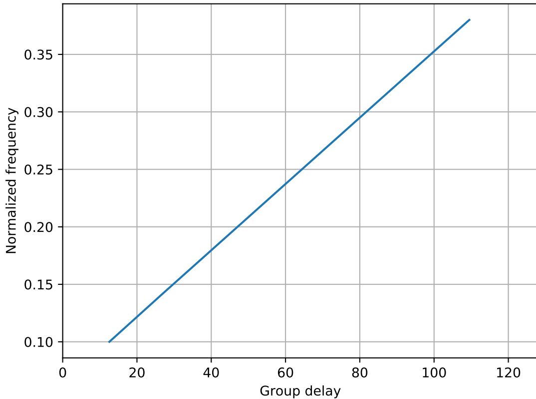
Group delay estimation of linear chirp
