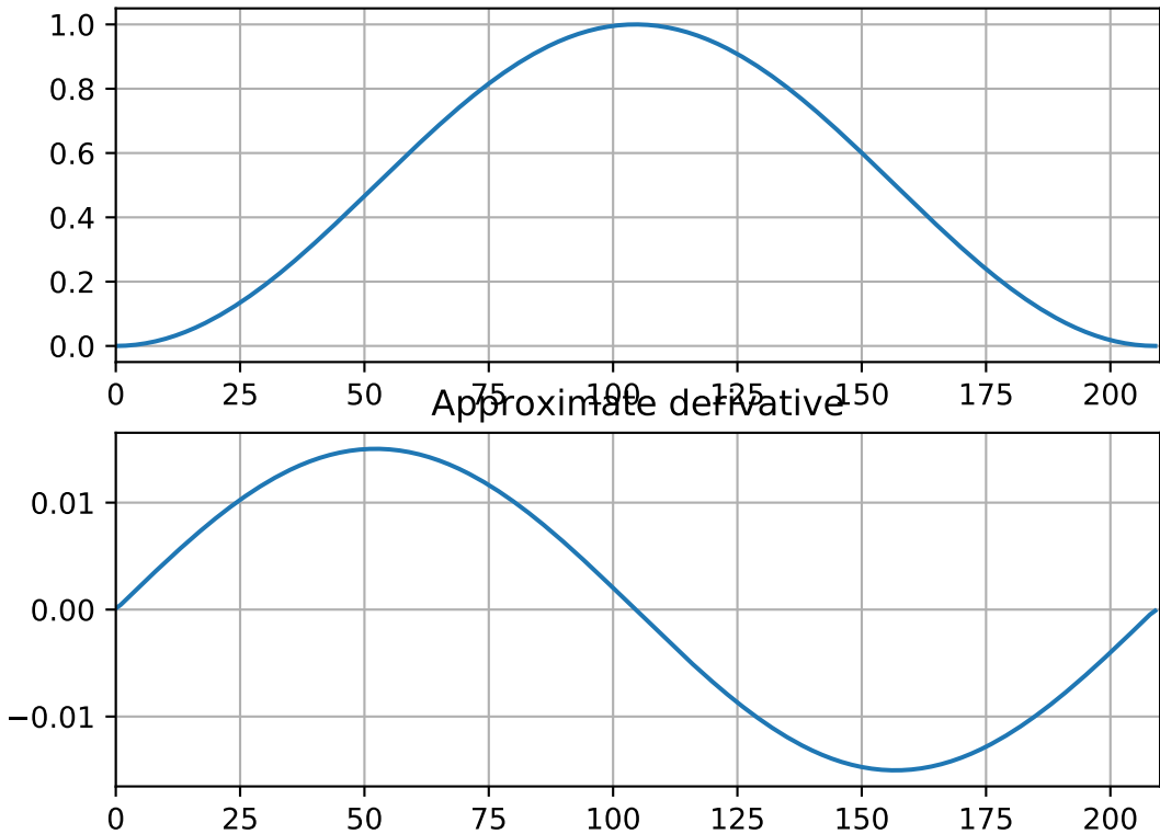
Hanning window
