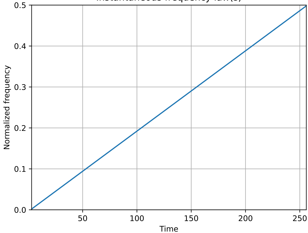
Instantaneous frequency law(s)
